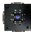
Multuser interface
