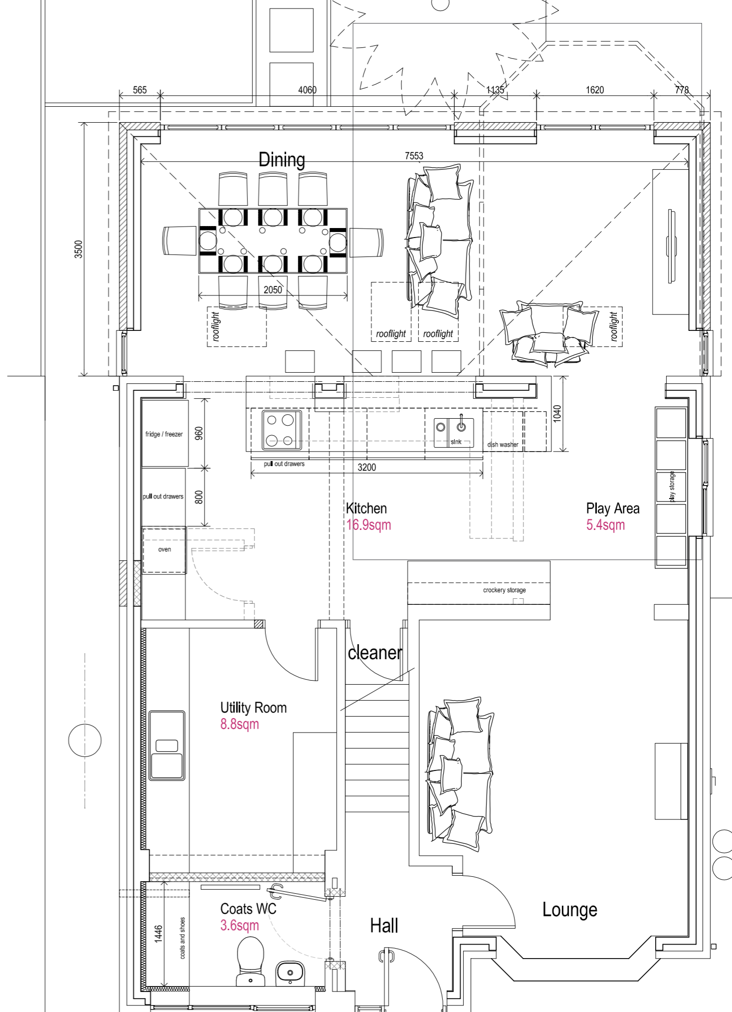
GROUND FLOOR PLAN - proposed
