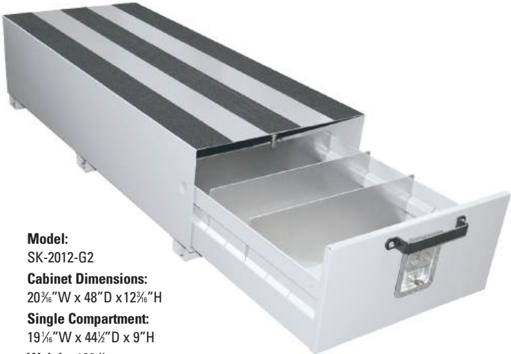
Recessed front conveyor rollers support up to 400 lbs. per drawer.
